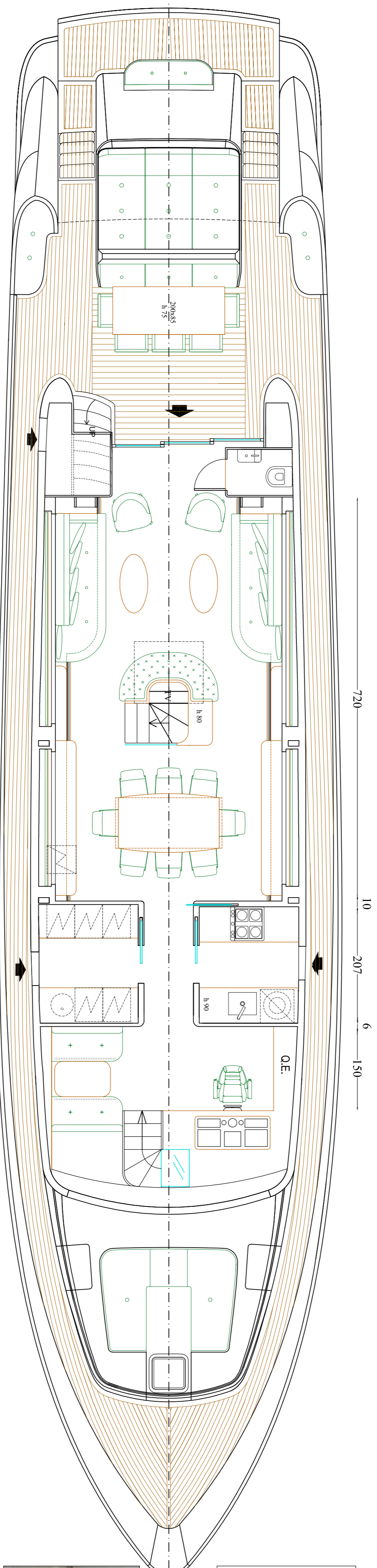
MAIN DECK
