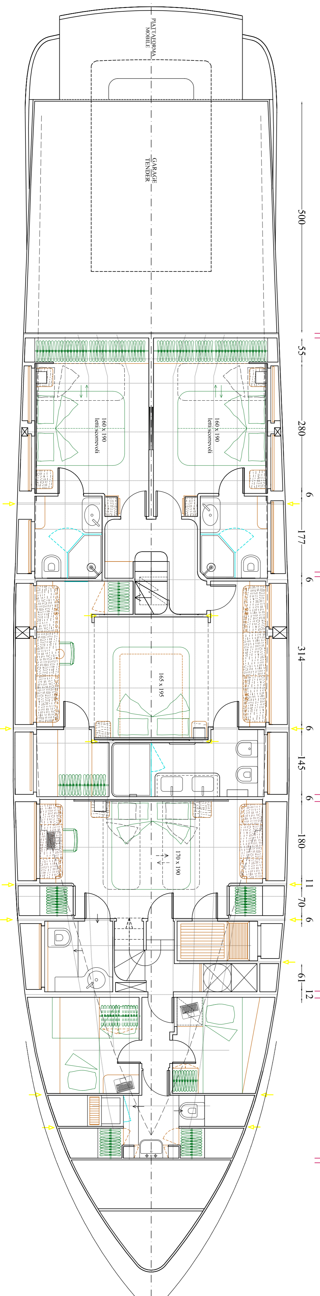
LOWER DECK
